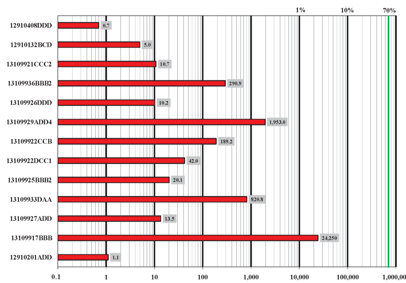
Figure 1. Graph depicting the relative relationship and absolute maximum values of flame-ionization detector (FID) instrument responses from selected wells in Bowman County. FID results for each well are presented in order of field screening occurrence from top to bottom. Values shown are those reported from the ground-water/air interface (GWI) (as CH 4 in ppm). The concentration of methane typical in commercial natural gas is highlighted by the vertical green line at 70%.
