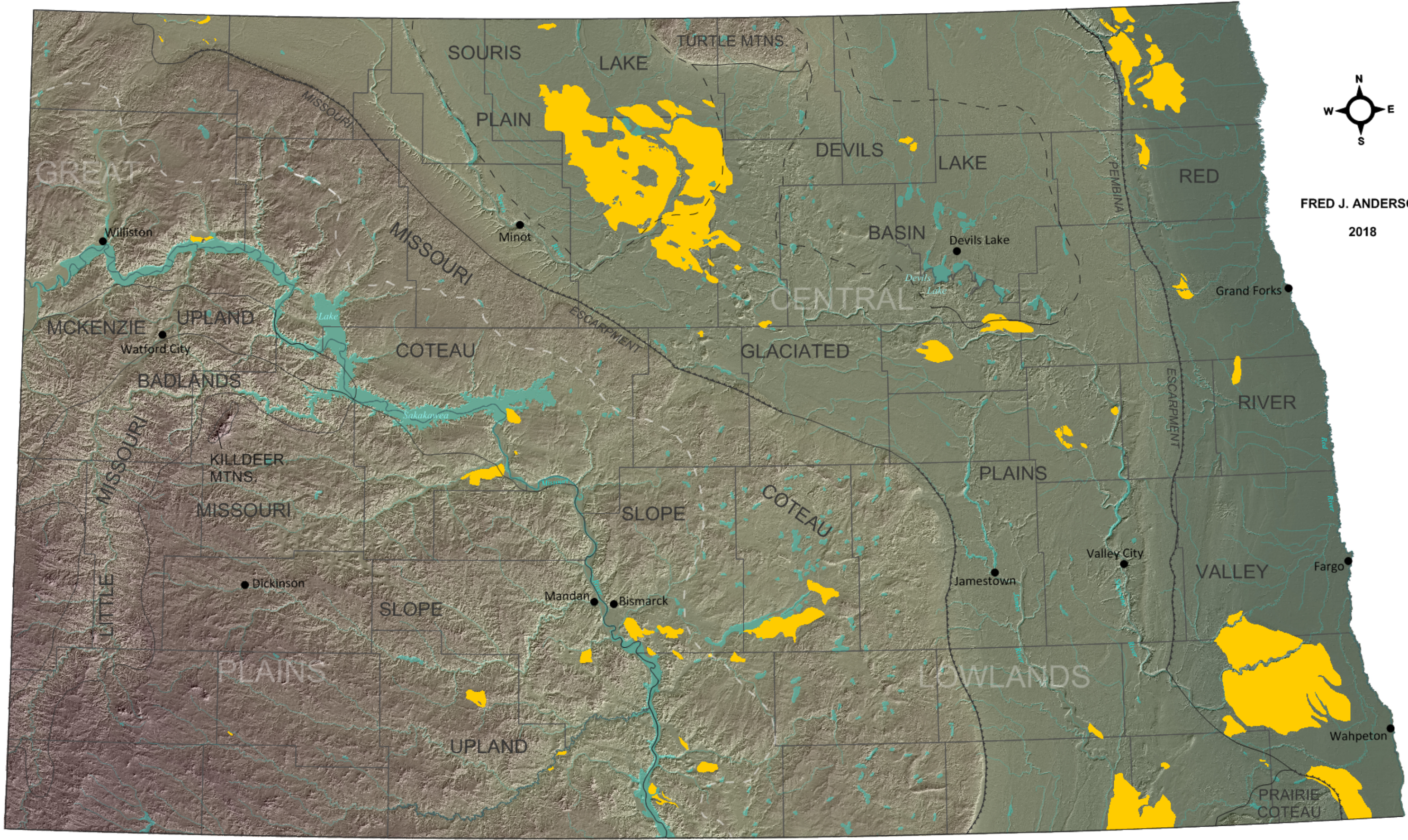
North Dakota's major physiographic regions are depicted with shaded-relief imagery.
