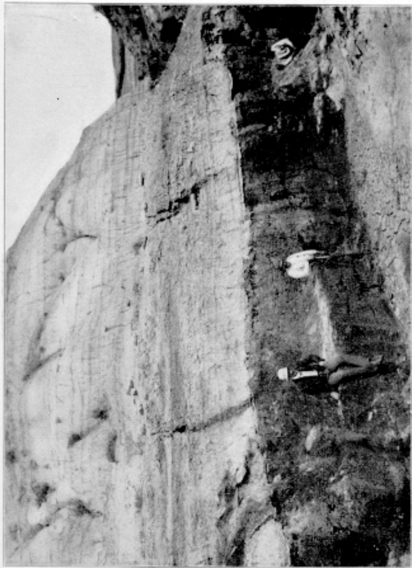
A Twelve-Foot Lignite Seam Near Williston, the Lower Portion Not Exposed, Showing the Laramie Clays With Rows of Concretions in the Bare Slopes Above.
