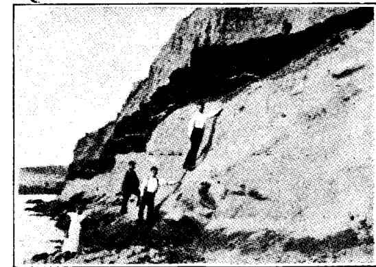
Lignite on the Missouri River west of Washburn.
