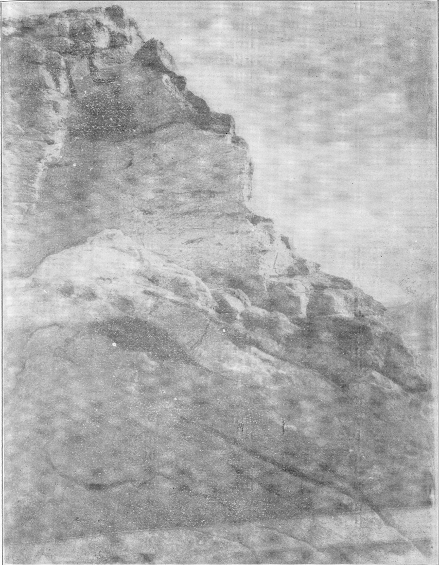
Sandstone at the Top of Sentinel Butte.
