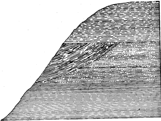
Fig. 1. Peculiar bedding in Laramie clays.
