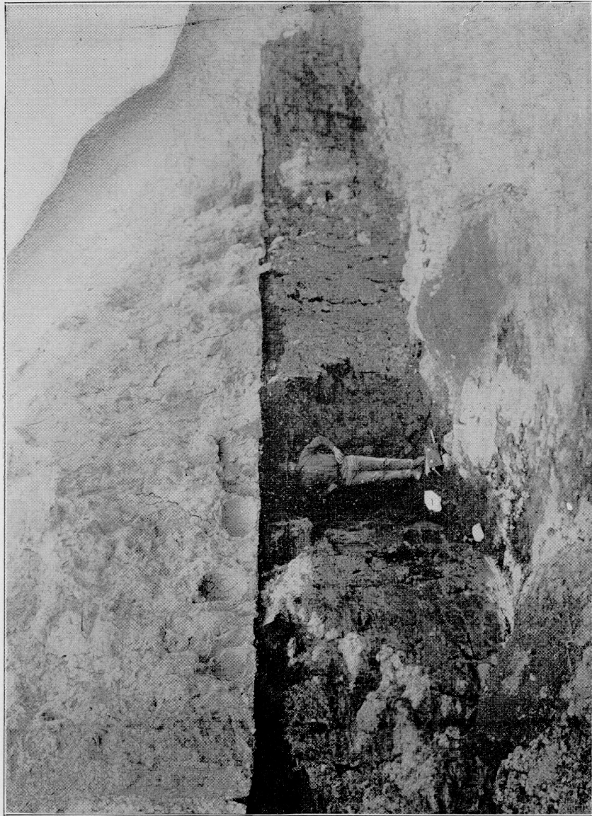
Part of an Eleven-Foot Seam Ten Miles Southwest of Velva; the Hanchett Mine.
