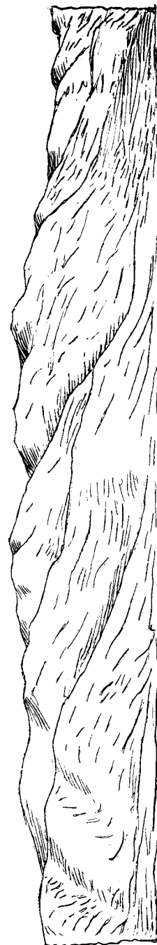
Fig. 15. Morainic hills west of Devils lake.
