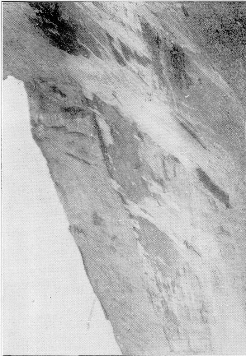
A Twenty-Foot Lignite Seam Outcropping in Township 133, Range 104, Section 20.
