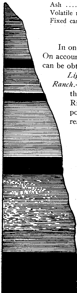
Fig. 6. Section thirty miles south of Medora at the 777 ranch, showing lignite seams.
