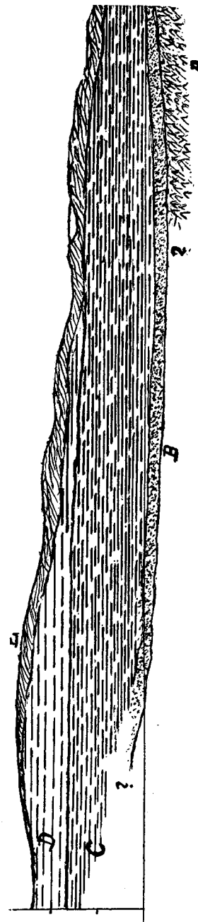
Fig. 17. Section showing water bearing strata.
