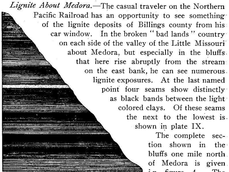
Fig. 4. A section showing the lignite seams in the bluffs at Medora.
