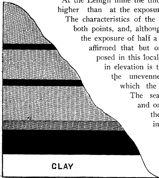
Fig. 12. Section at the Lehigh mine.
