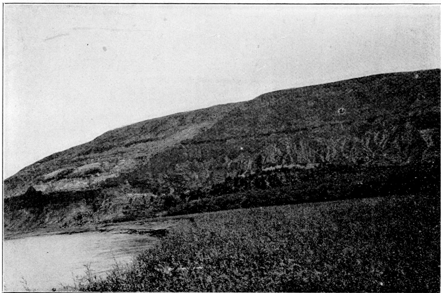
Bluffs on the Missouri, Three Miles Southeast of Williston, Showing Six Coal Seams.
