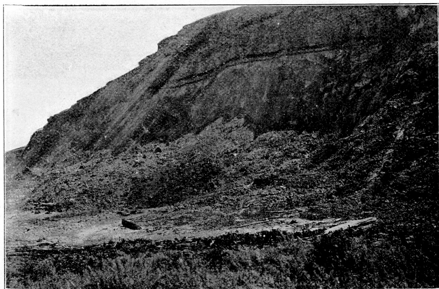
A Nearer View of the Above, Showing the Portion to the Left Only.
