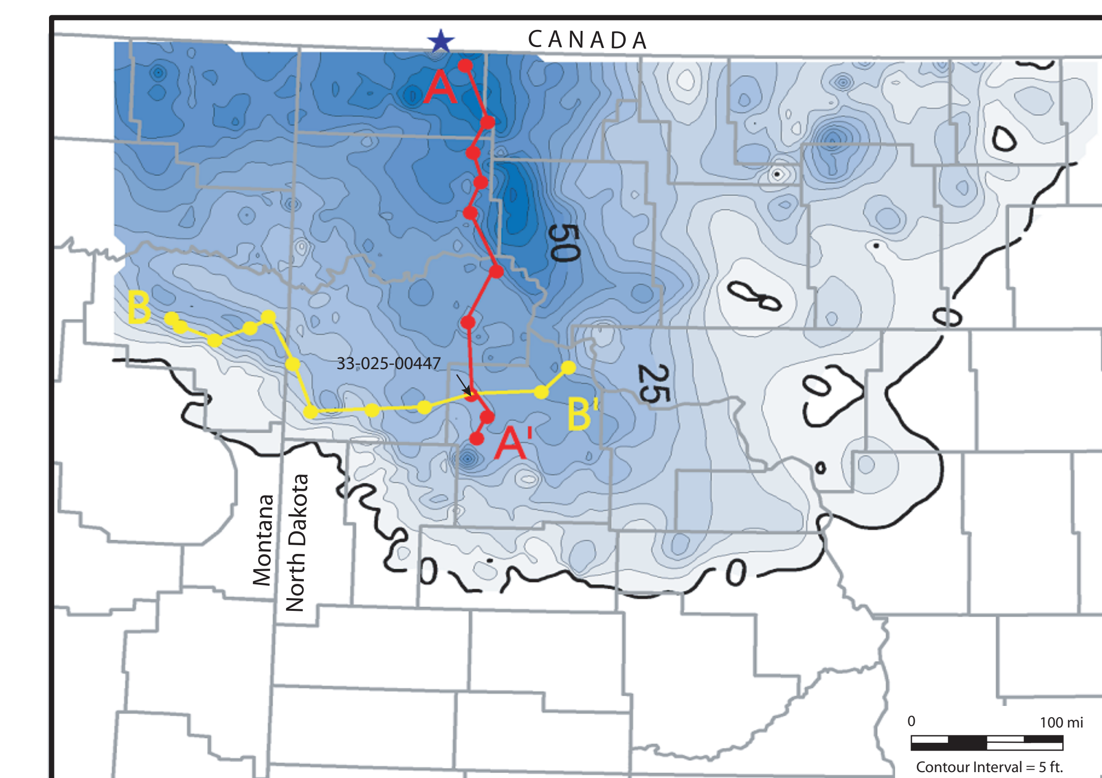
Lines of Cross-Section Isopach of the Middle Member of the Bakken Formation
