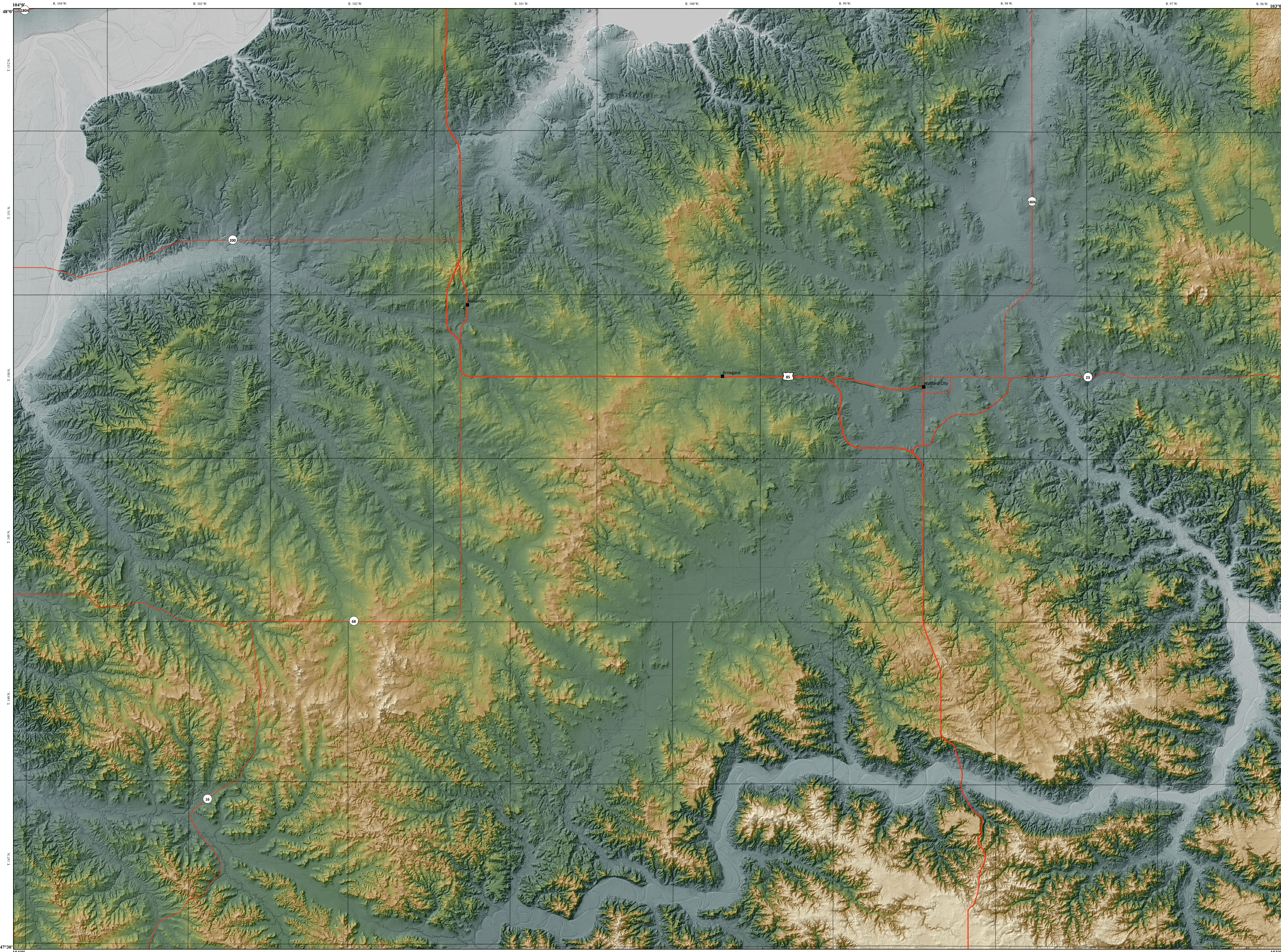
Watford City 100K Sheet, North Dakota
