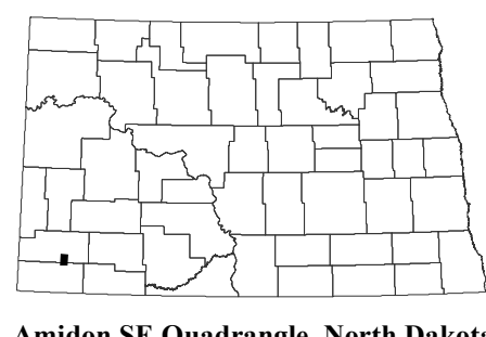
Amidon SE Quadrangle, North Dakota
