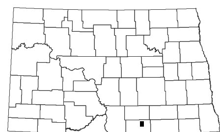
Ashley NE Quadrangle, North Dakota
