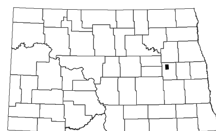
Binford Quadrangle, North Dakota
