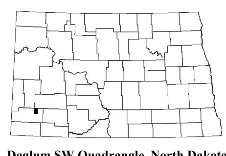
Daglum SW Quadrangle, North Dakota
