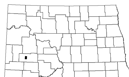
Dickinson South Quadrangle, North Dakota
