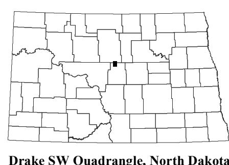
Drake SW Quadrangle, North Dakota
