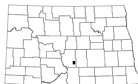
Driscoll Quadrangle, North Dakota
