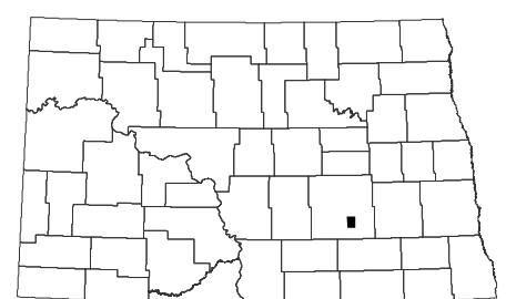
Eldridge SE Quadrangle, North Dakota
