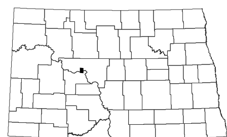
Emmet SE Quadrangle, North Dakota
