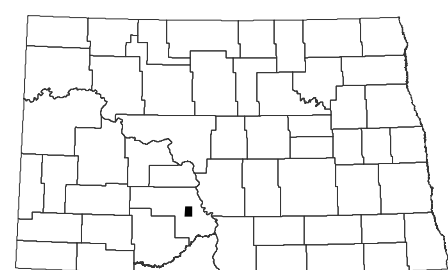
Fallon NE Quadrangle, North Dakota
