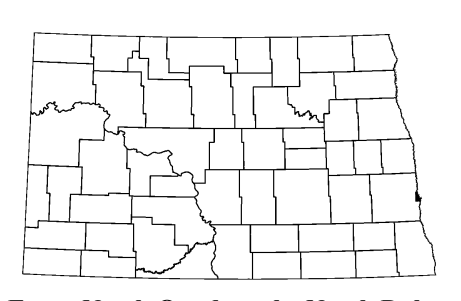
Fargo North Quadrangle, North Dakota
