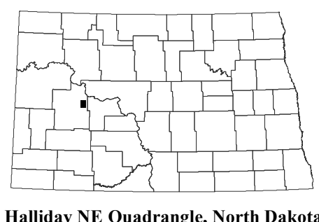
Halliday NE Quadrangle, North Dakota
