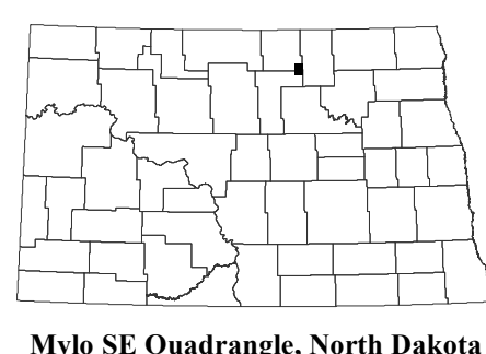
Mylo SE Quadrangle, North Dakota
