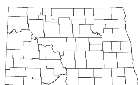
Northgate Quadrangle, North Dakota
