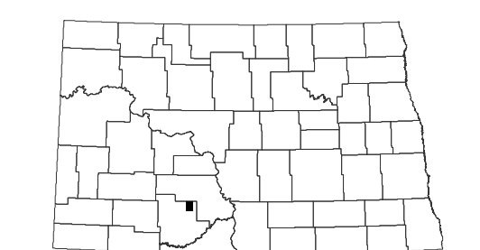
Otter Creek West Quadrangle, North Dakota
