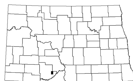
Raleigh Quadrangle, North Dakota
