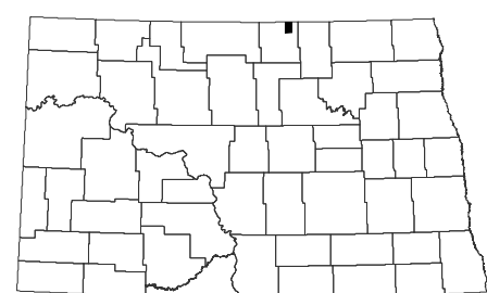
Saint John Quadrangle, North Dakota
