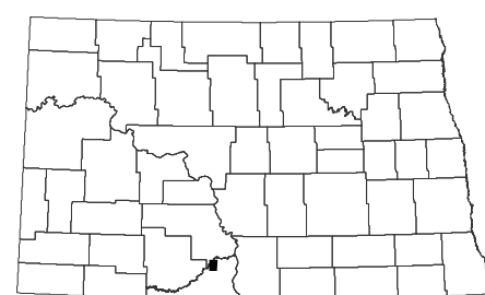
Solen SW Quadrangle, North Dakota
