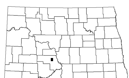
Sweet Briar Quadrangle, North Dakota
