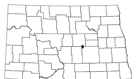
Sykeston SW Quadrangle, North Dakota
