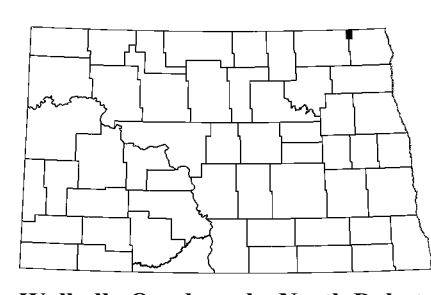
Walhalla Quadrangle, North Dakota
