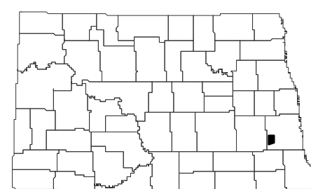
Alice Quadrangle, North Dakota
