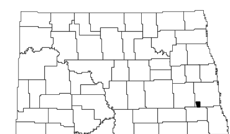
Enderlin North Quadrangle, North Dakota
