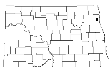
Minto Quadrangle, North Dakota
