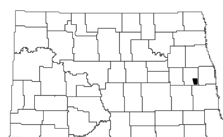
Hope SE Quadrangle, North Dakota
