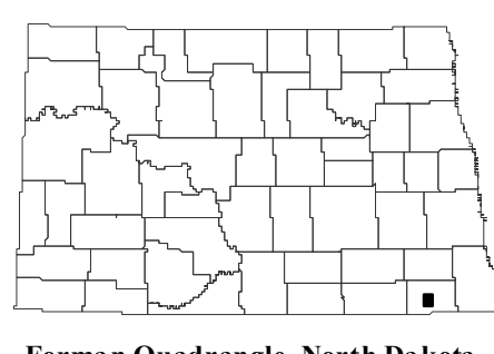
Forman Quadrangle, North Dakota
